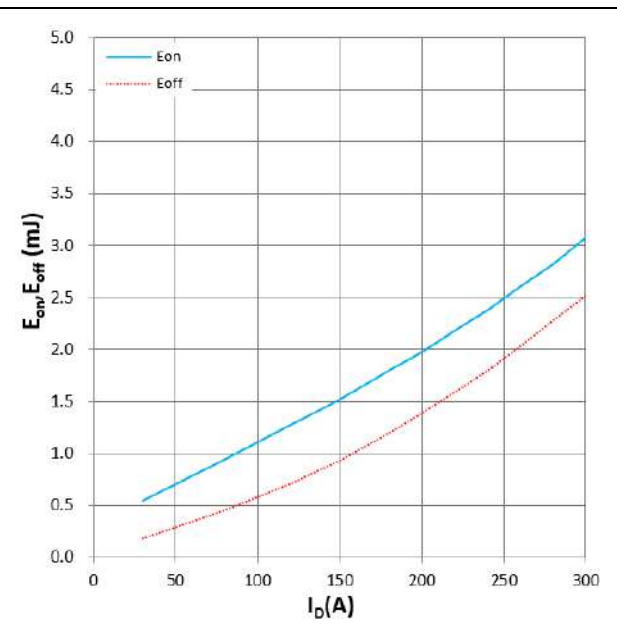
Figure 14. Eon, Eoff vs IDS Tj = 25°C, RG = 3.3mΩ, VGS = +18V/-4V
