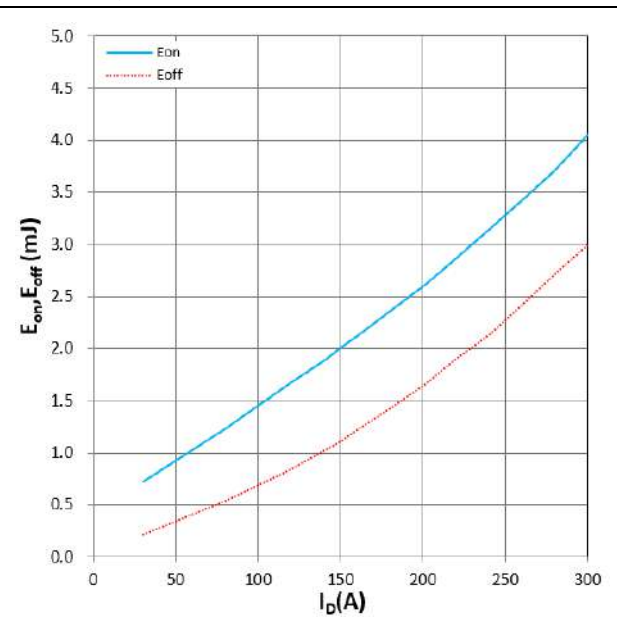
Figure 16. Eon, Eoff vs IDS Tj = 150°C, RG = 3.3mΩ, VGS = +18V/-4V
