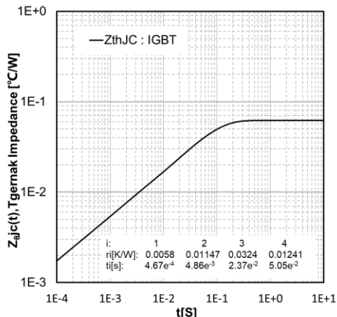
Fig.11 Transient thermal impedance IGBT, Inverter
