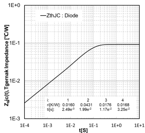
Fig.12 Transient thermal impedance Diode, Inverter
