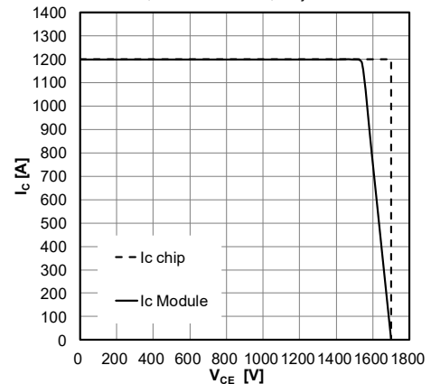
Fig.6 Reverse bias safe operating area (RBOSA), IGBT, Inverter I_C = f(V_{CE}) R_{Goff} = 1.0 \Omega , V_{GE} = \pm 15V , T_{vj} = 175^\circ C
