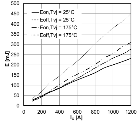
Fig.4 Switching losses, IGBT, Inverter E = f(I_C) R_{Goff} = 1.0 \Omega , R_{Gon} = 1.0 \Omega , V_{CE} = 900V , V_{GE} = \pm 15V
