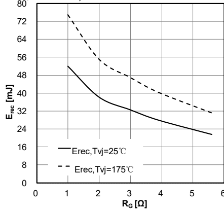
Fig.7 Switching losses, Diode, Inverter
