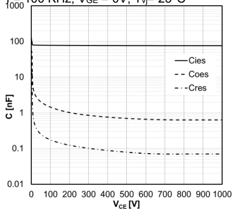
Fig.3 Capacity characteristic, IGBT, Inverter C = f(V_{CE}) f = 100 KHz , V_{GE} = 0V , T_{vj} = 25^\circ C
