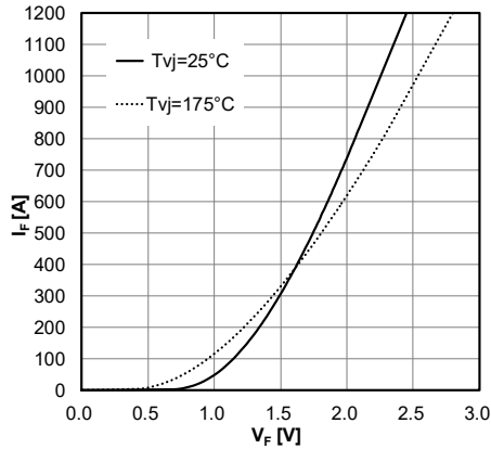
Fig.9 Forward characteristic, Diode, Inverter
