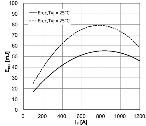
Fig.10 Switching losses, Diode, Inverter
