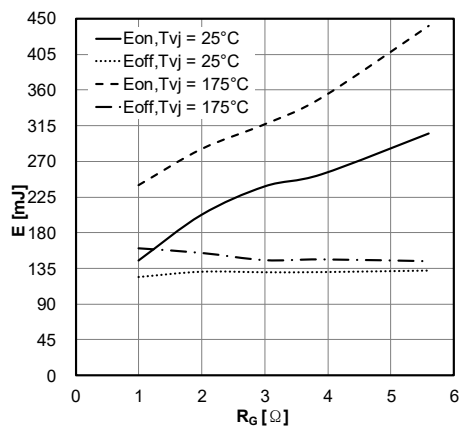
Fig.5 Switching losses, IGBT, Inverter E = f(R_G) I_C = 600A , V_{CE} = 900V , V_{GE} = \pm 15V
