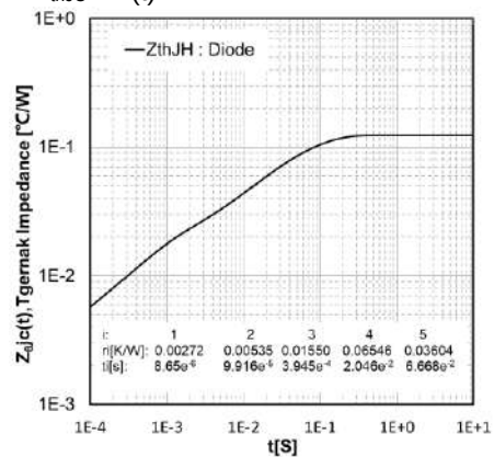
Fig.13 Transient thermal impedance Diode, Inverter
