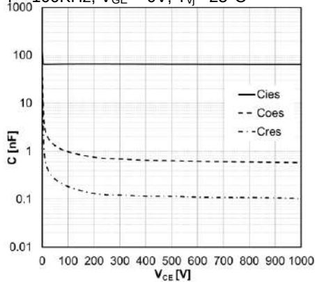
Fig.7 Capacity characteristic, IGBT, Inverter
