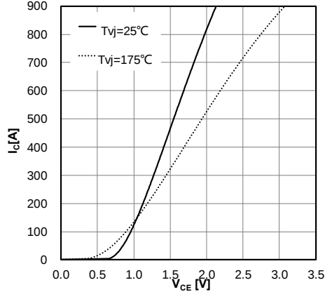
Fig.1 Typical Output Characteristic, IGBT, Inverter I_C = f(V_{CE}) / (terminal)
