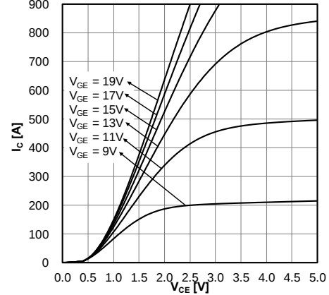
Fig.2 Typical Output Characteristic, IGBT, Inverter I_C = f(V_{CE}) / (terminal)
