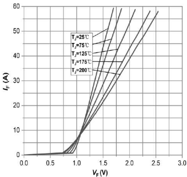
Figure 1: Forward Characteristics
